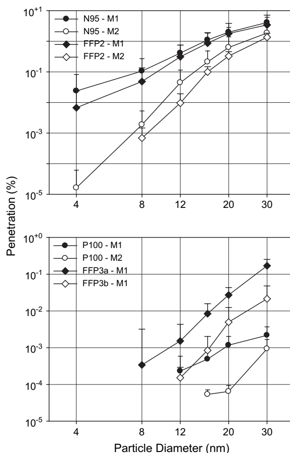
Fig. 3. Percentage penetrations of monodisperse silver particles (4–30 nm) through N95, FFP2, P100 and FFP3 FFR from two different manufacturers (M1 and M2) at 85 \text{ l min}^{-1} flow rate (MAT-1 method). Error bar indicates the 95% confidence interval ( n = 5 ).
