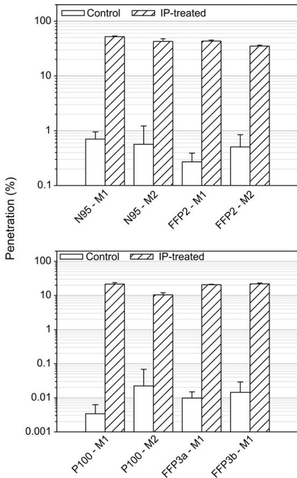
Fig. 6. Percentage penetration levels of 238 nm MMD polydisperse aerosols (PAT method) for different FFR types and manufacturers (M1 and M2) before (control) and after isopropanol treatment (IP-treated) at 85 l min -1 flow rate. Error bar indicates the 95% confidence interval ( n = 5 ).
